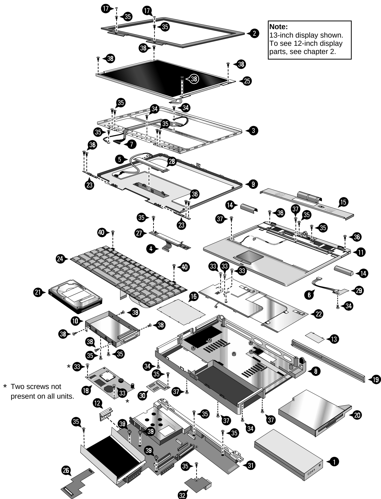
Figure 4-1. Exploded View
